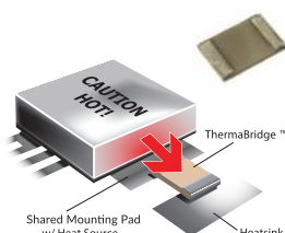
Thermal Bridge
